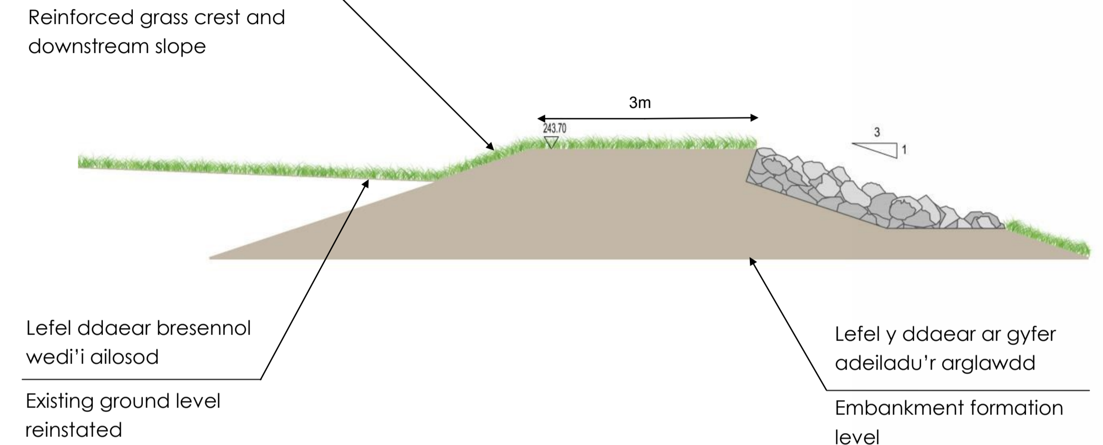
Rhan arferol, arglawdd cronfa ddŵr arfaethedig Typical section, proposed reservoir embankment
