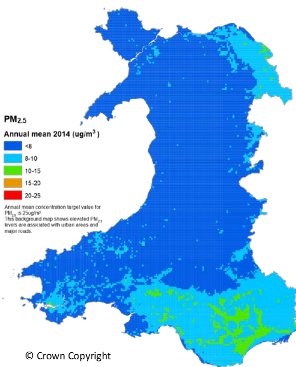
Figure 3.4 PM 2.5 concentrations in Wales 41 . [H]
