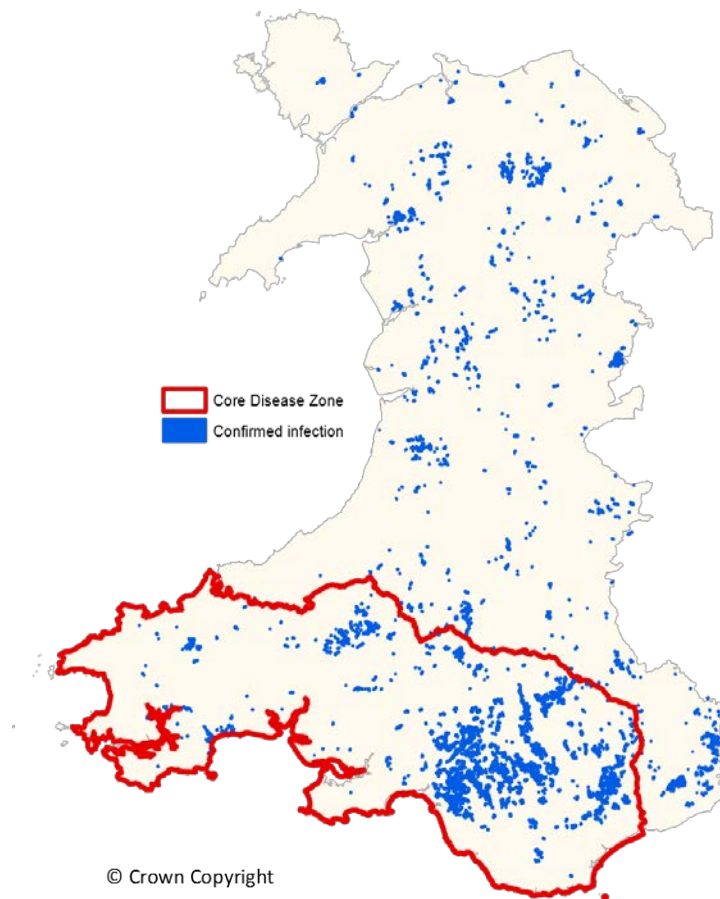
Figure 3.23 Distribution of Phytophthora ramorum in Wales in 2016 163 . [H]
