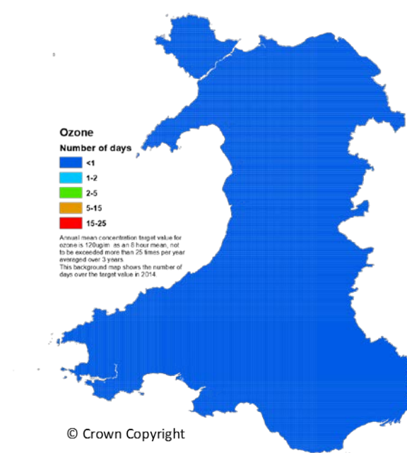
Figure 3.7 Number of days background ozone concentration was over target value in 2014 41 . [M]
